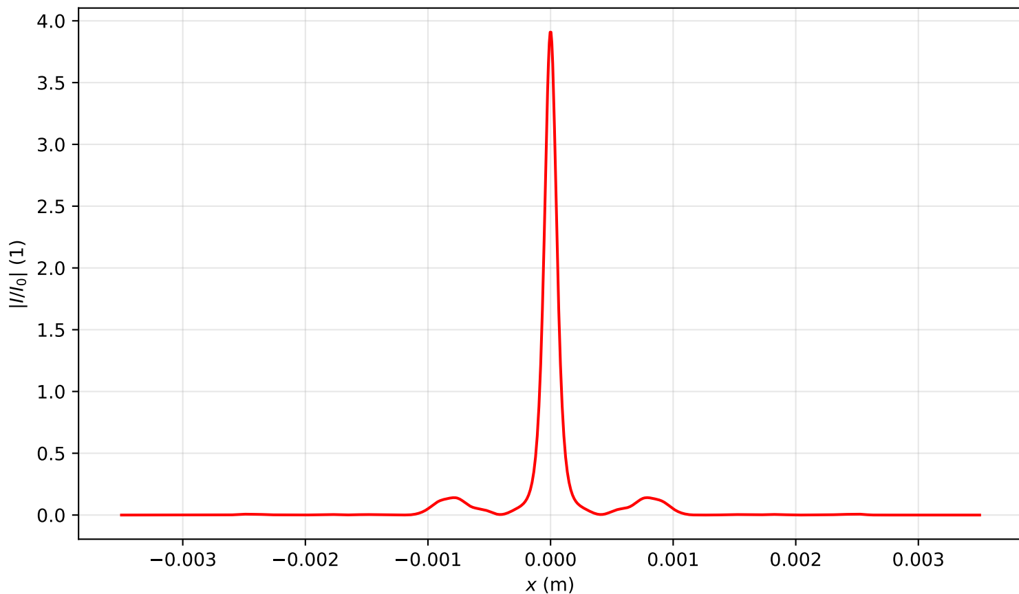
Intensity profile I(x, y = 0, z = 1.433)/I_0 , P_{in}=9.0P_{cr} , artificial time
